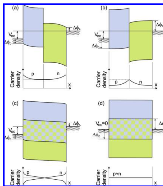
FIGURE 6. Schematic band diagrams and hole (p) and electron (n) carrier densities at open-circuit voltage ( V_{OC} ) conditions vs position ( x ) within the device for (a, b) planar heterojunctions and (c, d) bulk heterojunctions. The carrier injection barriers ( \Delta\phi ) at the contacts are either (a, c) small or (b, d) large.
